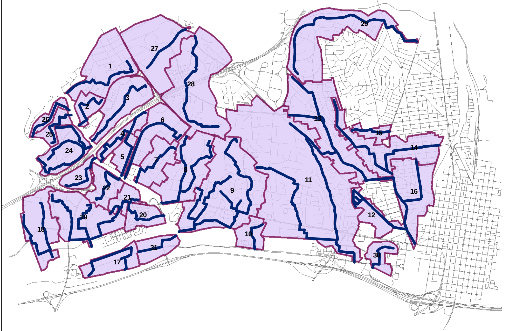
FIGURE 5-1 SANITARY SEWER CAPACITY ANALYSIS Sanitary Sewer Master Plan
