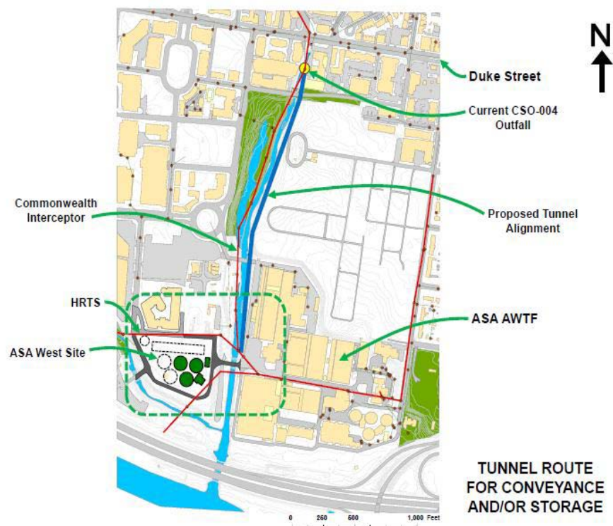
FIGURE 7-5 CSO RELOCATION AND STORAGE
